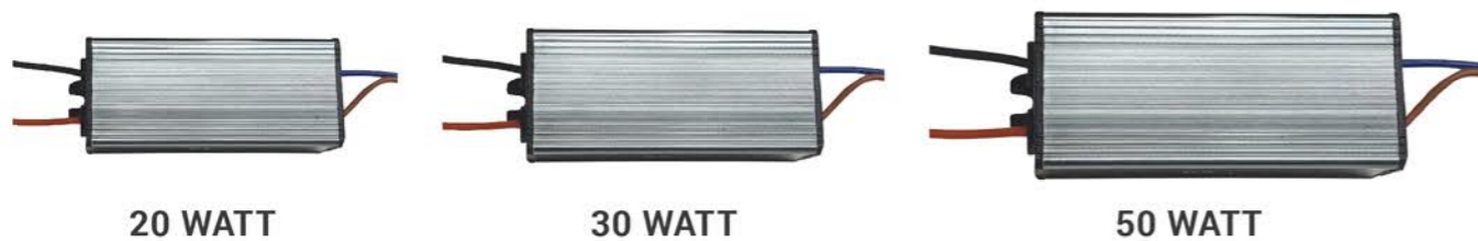
WATER PROOF DRIVER 20 TO 50 WATT
