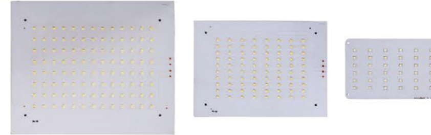
FLOOD & STREET LIGHT PCB 18 TO 200 WATT
